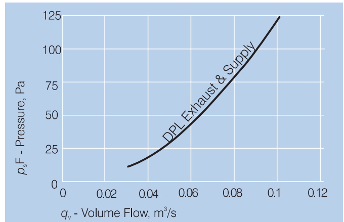
Slimfit Louvre Grille (Model No: DPL150)
