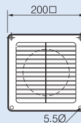
Slimfit Louvre Grille (Model No: DPL150)
