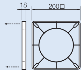
Spacer Plate (Model No: DPS150)
